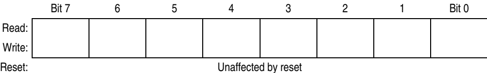
Figure 4-2. Accumulator (A)
