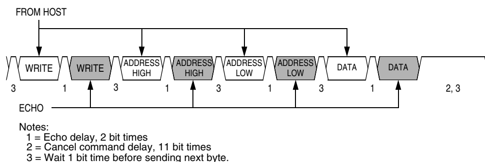
Figure 8-6. Write Transaction
